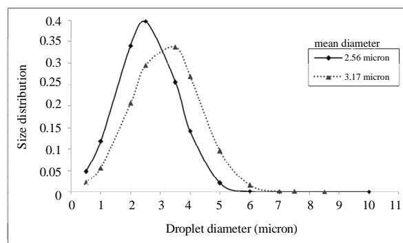
Figure 3. The effect of changing surfactant on the DSD: emulsion with tween80 (dash line); emulsion
