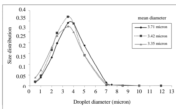
Figure 11. The effect of power of homogenizer on the DSD: emulsions with Triton x-100 (0.00225ml/100ml solution) with 480W power of homogenizer (grey solid line); with 960W power of homogenizer (dash line); with 2240W power of homogenizer (black solid line)
