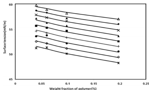
Figure 4. Surface tension of PEG 6000 in water at different temperatures and concentrations: ■, Δ,T=298.15 K; ◆,T=303.15 K; ×,T=308.15 K; ▲,T=313.15 K; ■,T=318.15 K; +,T=323.15 K; ●,T=328.15 K; ◇,T=333.15K; *,T=338.15; - Neural network.
