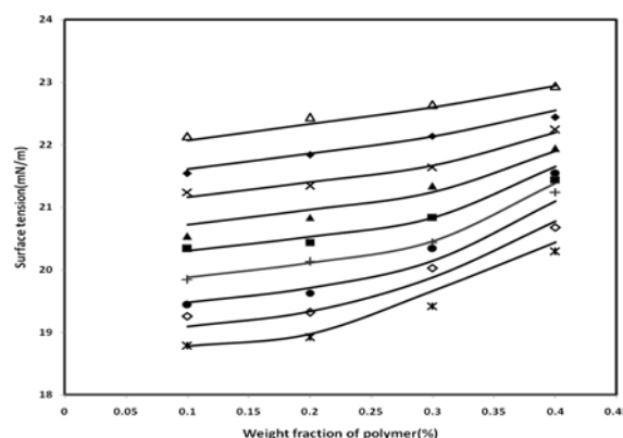
Figure 5. Surface tension of PPG 2000 in ethanol at different temperatures and concentrations: ■, Δ,T=298.15 K; ◆,T=303.15 K; ×,T=308.15 K; ▲,T=313.15 K; ■,T=318.15 K; +,T=323.15 K; ●,T=328.15 K; ◇,T=333.15K; *,T=338.15; - Neural network.
