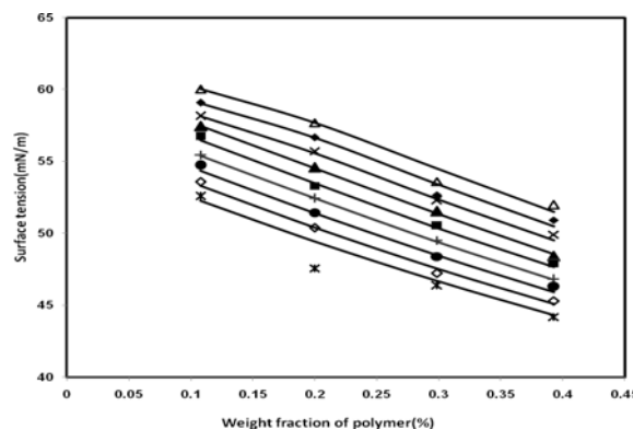
Figure 3. Surface tension of PEG 300 in water at different temperatures and concentrations■, Δ,T=298.15 K; ◆,T=303.15 K; ×,T=308.15 K; ▲,T=313.15 K; ■,T=318.15 K; +,T=323.15 K; ●,T=328.15 K; ◇,T=333.15K; *,T=338.15; - Neural network.
