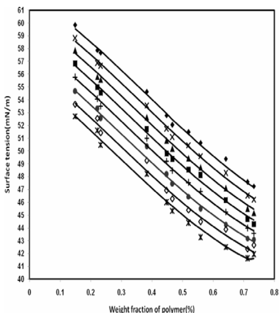
Figure 2. Surface tension of PEG 200 in water at different temperatures and concentrations : ,■, Δ,T=298.15 K; ◆,T=303.15 K; ×,T=308.15 K; ▲,T=313.15 K; ■,T=318.15 K; +,T=323.15 K; ●,T=328.15 K; ◇,T=333.15K; *,T=338.15; - Neural network.
