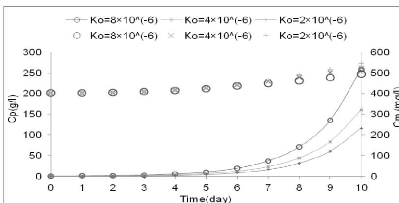
Figure 7. Changes in substrate (line style) and biomass (dot style) based on oxygen half-saturation coefficient ( K_o )
