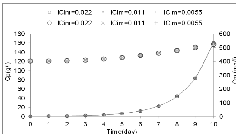
Figure 6. Changes in substrate (line style) and biomass (dot style) based on production rate of endogenous substrate ( IC_{im} )
