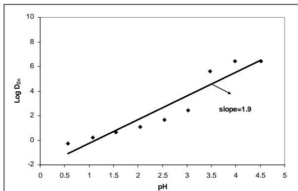
Figure 3. Log D_{Zn} vs. pH in Zn extraction using [D2EHPA] = 40 vol. %, O: A=1 and feed solution: [Zn 2+ ] = 25g/L, [Ni 2+ ] = 1.5g/L and [Cd 2+ ] < 20mg/L
