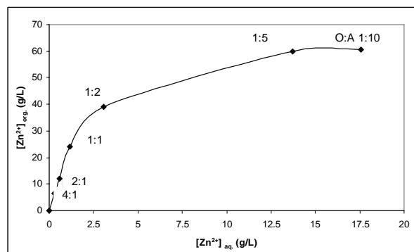
Figure 4. Distribution isotherm for extraction of Zn at pH = 2.5-3 and [D2EHPA] = 40 vol.%, from feed solution: [Zn 2+ ] = 25g/L, [Ni 2+ ] = 1.5g/L and [Cd 2+ ] < 20mg/L
