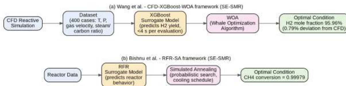
Figure 8. Optimization frameworks for the hybrid reforming-process: (a) CFD–XGBoost–WOA for optimizing the yield of \text{H}_2 and (b) RFR–SA for optimizing \text{CH}_4 -conversion.
