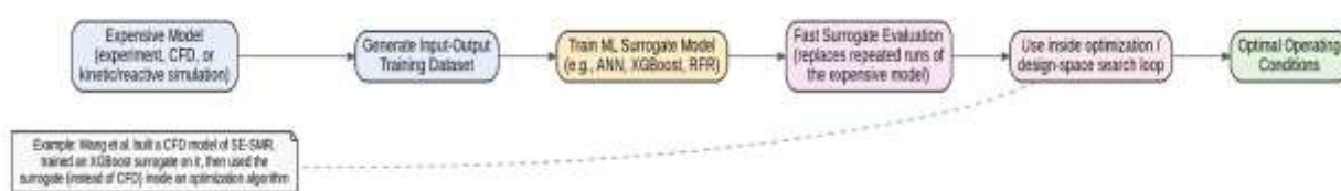
Figure 7. General surrogate-model framework in which experimental or simulation data train an ML model that replaces repeated high-cost process calculations during analysis or optimization.
