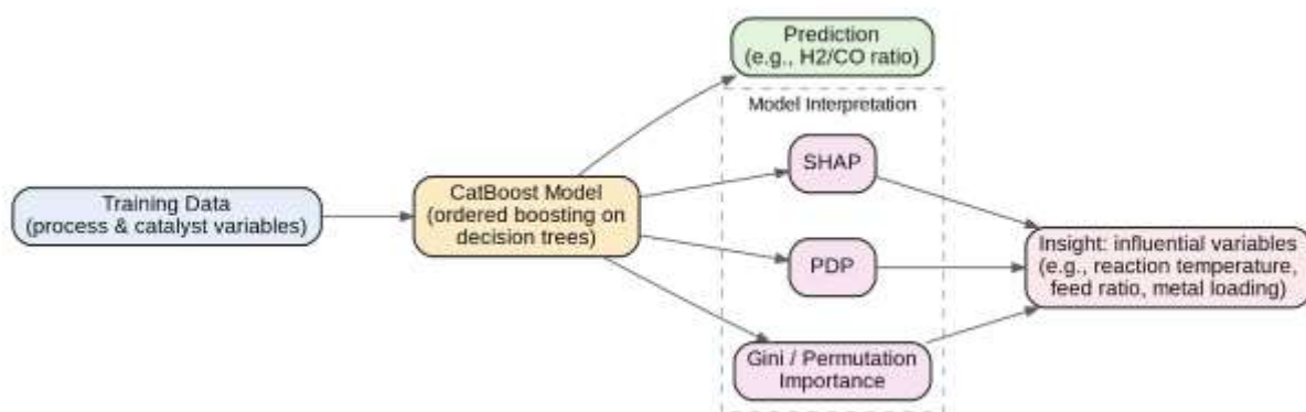
Figure 6. CatBoost prediction framework combined with explainable ML tools (SHAP, PDP, and feature importance) for evaluating the statistical contribution of reforming-process inputs.
