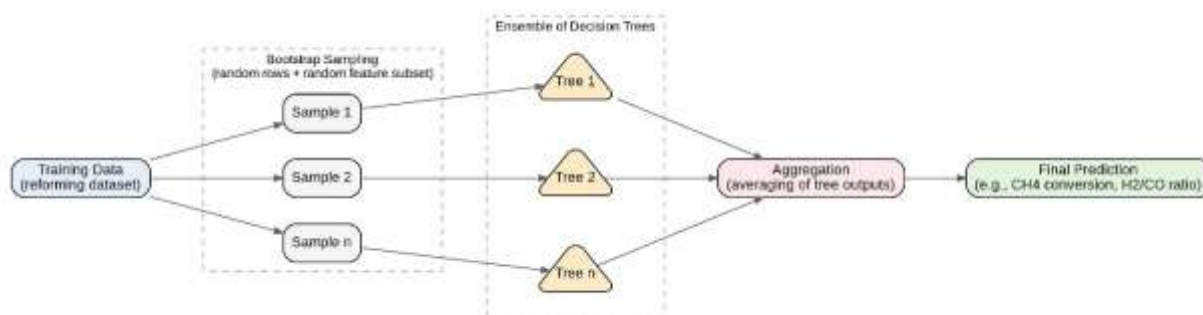
Figure 2. Structure of the Random Forest regression framework, illustrating bootstrap sampling, decision-tree construction, and aggregating tree predictions for estimating the process output.
