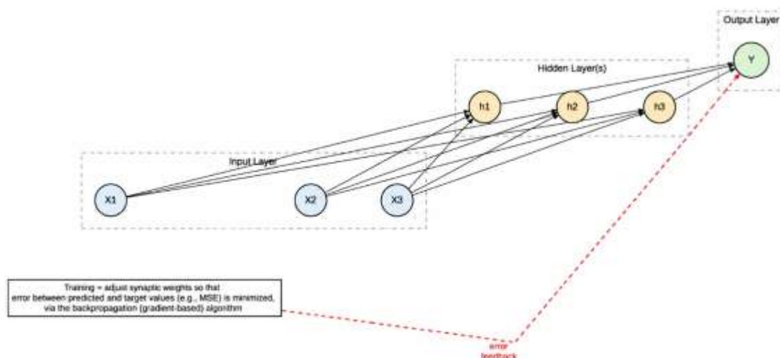
Figure 1. General structure of an artificial neural network (MLP), showing the input, hidden, and output layers and the iterative weight-update process used during training.
